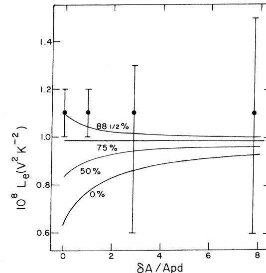
FIG. 1. Comparison of calculated and measured values of L_e for Pd and dilute Pd-Ni alloys. A is the coefficient of the T^2 term in the electrical resistivity, and \delta A = A_{\text{alloy}} - A_{\text{Pd}} . Solid dots and error bars represent values of L_e extracted from the data. The 0% curve is the result of a calculation with the local-enhancement model of paramagnon scattering with \bar{I}_{\text{Pd}} = 0.9 , k_s = 0.9125 \times 10^8 \text{cm}^{-1} , and k_d = 2k_s . The other curves are the results of modifying the calculation by adding a concentration-independent amount of Baber scattering to the paramagnon scattering. The percentages indicate for each curve the amount of the total resistivity in pure Pd which is assumed to be Baber scattering.
